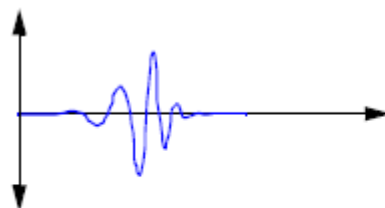
Wavelet function \psi(t)
